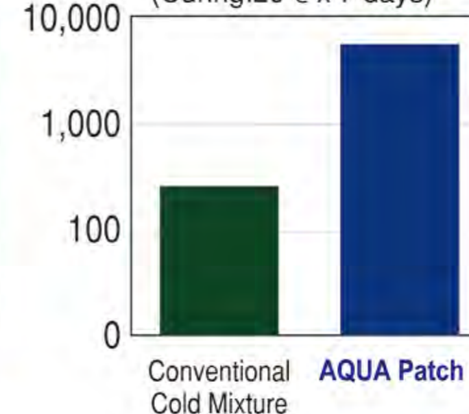
Wheel Traking Test (Curing: 20°C x 7 days)
