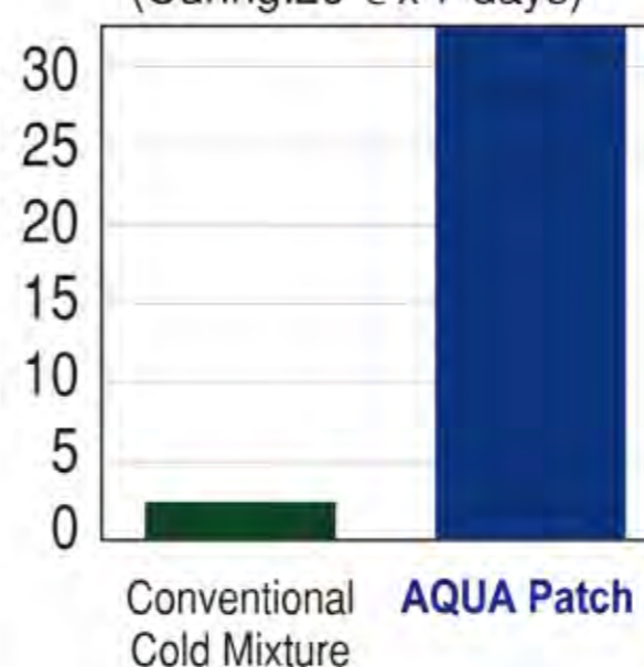
Marshall Stability Test (Curing: 20°C x 7 days)
